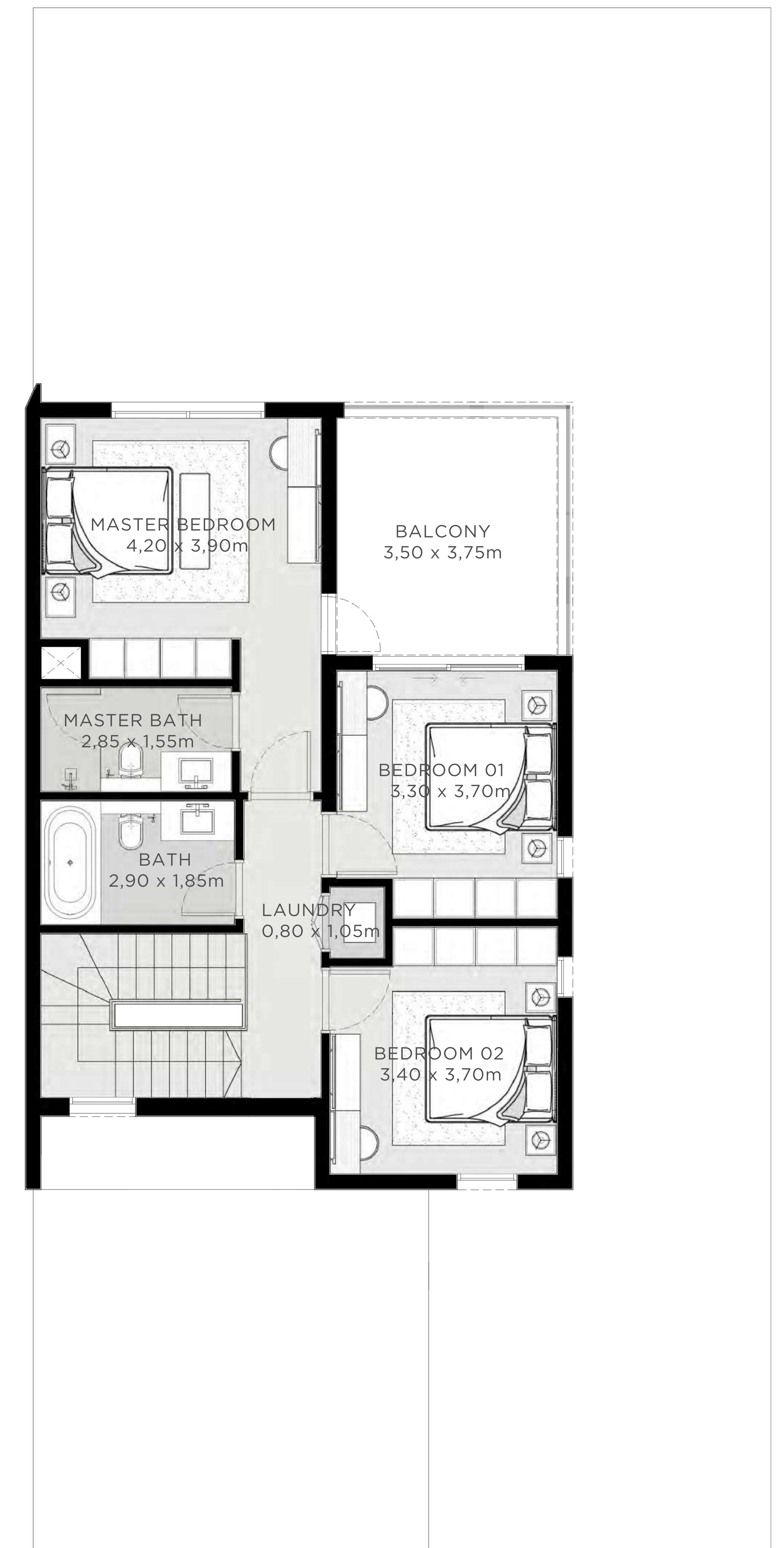
FIRST FLOOR
